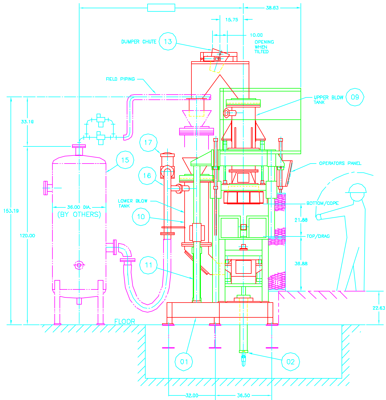
END VIEW
