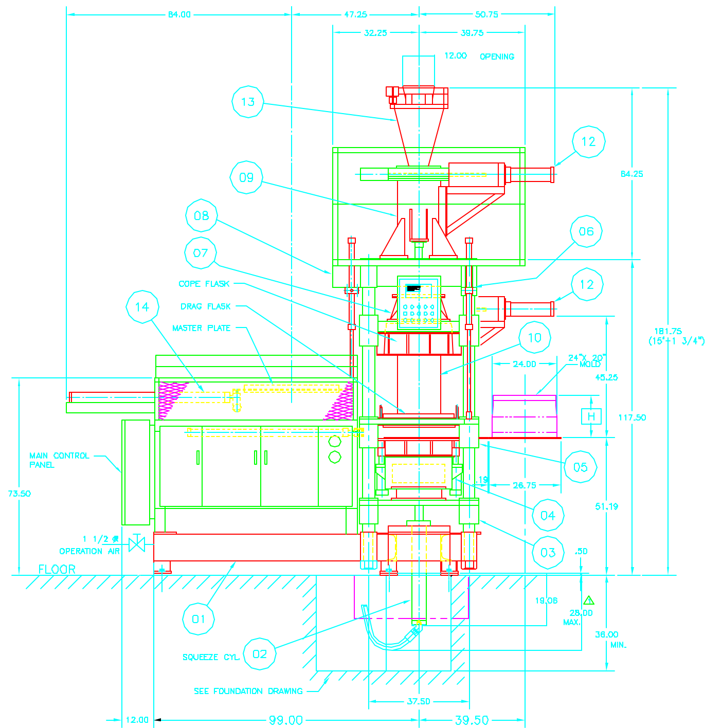
OPERATORS SIDE VIEW
