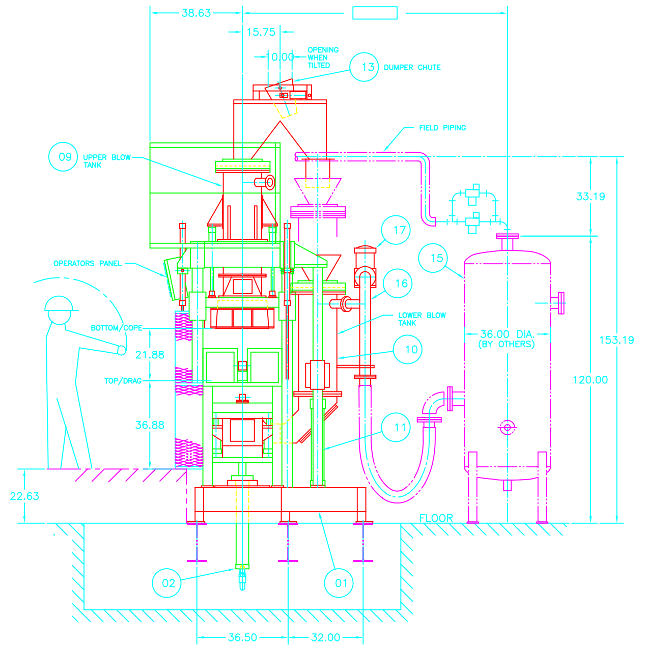
END VIEW
