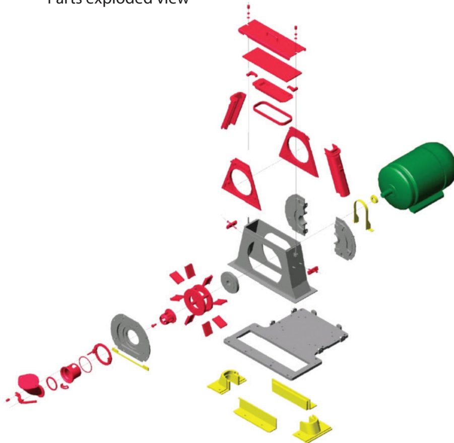
Parts exploded view
